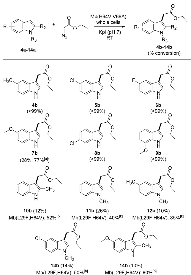
Scheme 2. Substrate scope for Mb(H64V,V68A)- and Mb(L29F,H64V)-catalyzed C–H functionalization of indoles. Reaction conditions: 2.5 mM indole derivative, 5 mM EDA, whole cells at OD 600 =20 in 50 mM phosphate buffer (pH 7), RT. [a] Using 75 \mu\text{M} Mb(H64V,V68A) in 50 mM phosphate buffer (pH 9) containing 10 mM Na 2 S 2 O 4 (sequential catalyst addition protocol). [b] As in [a] but using 85 \mu\text{M} Mb(L29F,H64V). Reported conversions are mean values from n \geq 2 experiments (SE < 10%).
