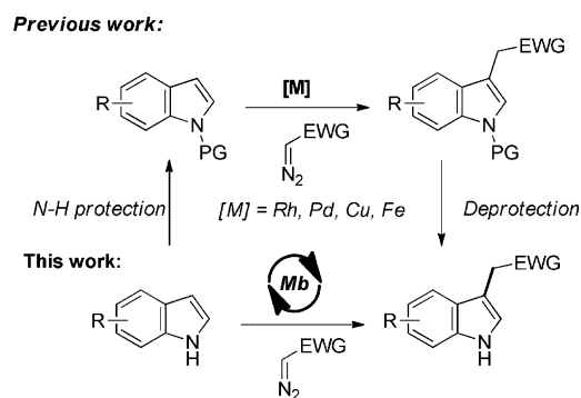
Scheme 1. Metal-catalyzed functionalization of N-protected indoles vs. biocatalytic functionalization of unprotected indoles reported herein.
